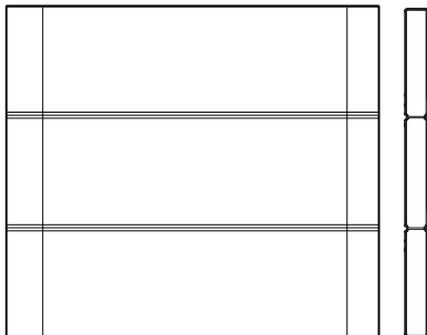
16135 - SLATE- ARDOISE - PIZARRA BOARD B - PLANCHE B - TABELRO B 9 1/2" (24.1 CM) - X4
