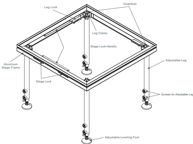
Tool-less leg lock
