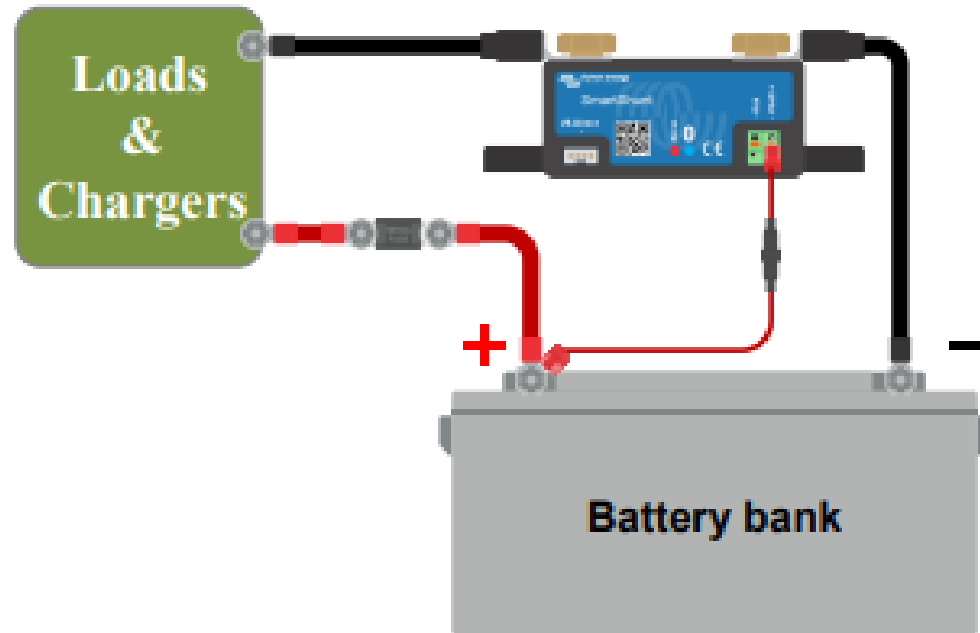
Basic battery monitor installation.
