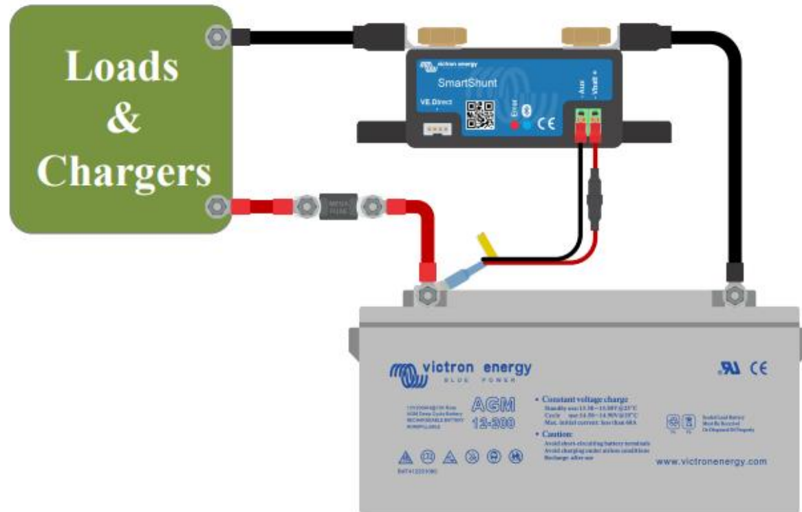
Battery monitor with auxiliary temperature sensing.
