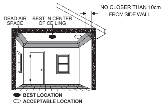
Figure 4: Recommended smoke-alarm mounting locations:
