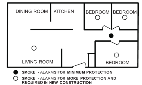
Figure 2: Recommended smoke-alarm protection for single-floor residence with more than one sleeping area:
