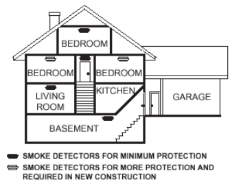
Figure 3: Recommended smoke-alarm protection for a multi-level residence:
