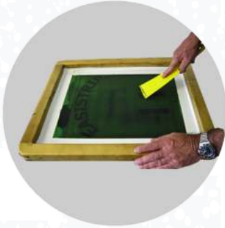
1. SCRAPE INK
