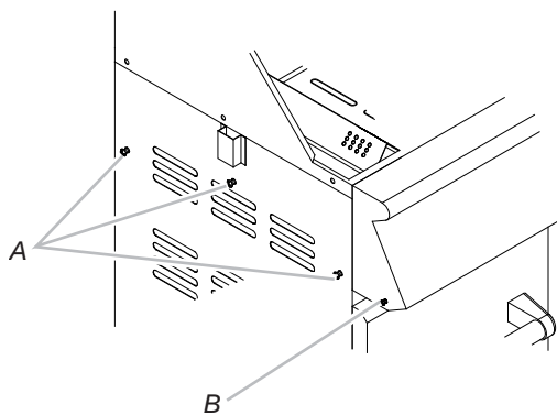
A. Grill side panel screws
