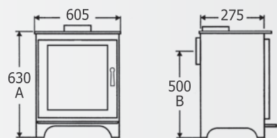
Long leg option dimensions
