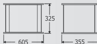
Bolt on log store shown with short leg option stove
