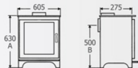
Long leg option dimensions
