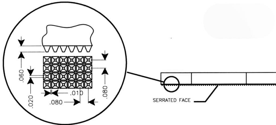
SERRATION DETAIL
