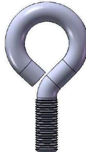
3/8"-16 X 3/4" DIA. I.D. X 2-1/2" L EYE BOLT QTY: 2
