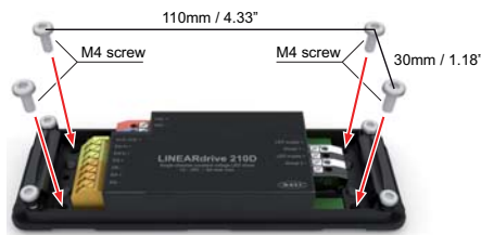
B Mounting the LED driver
