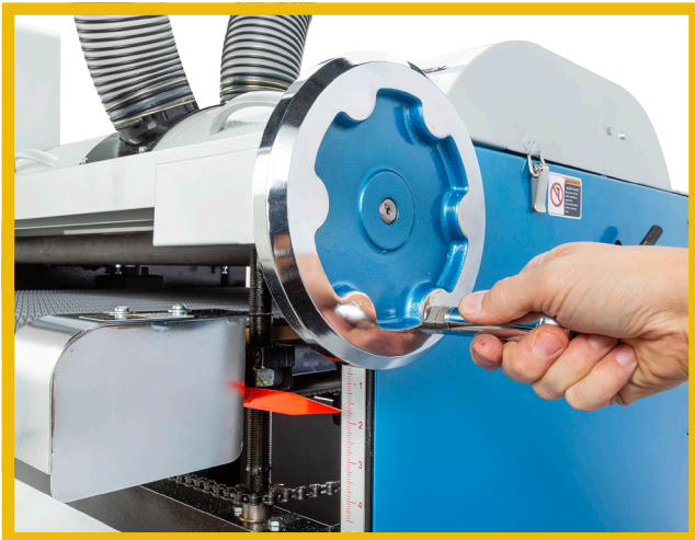
The table height hand wheel
