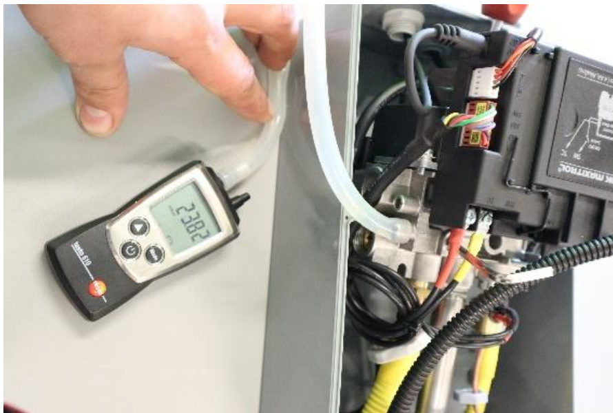
Testing pressure
