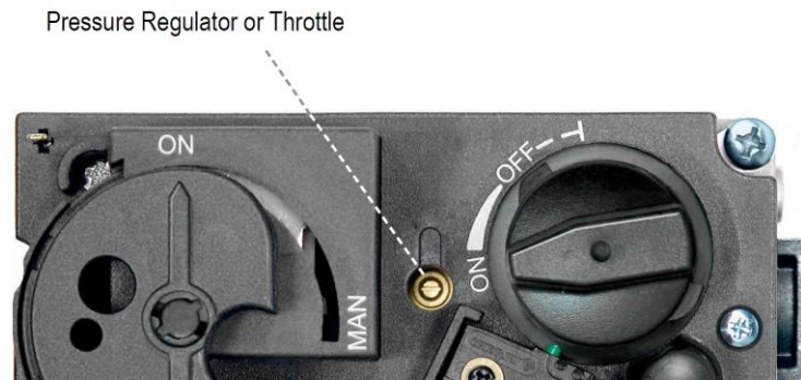
Outlet pressure adjustment
