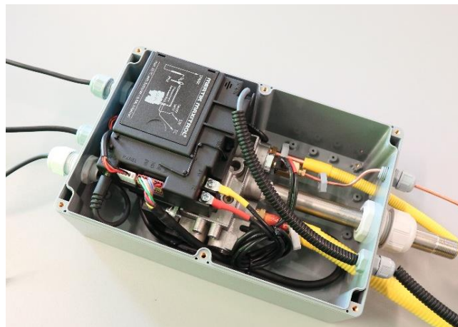
Valve box elements
