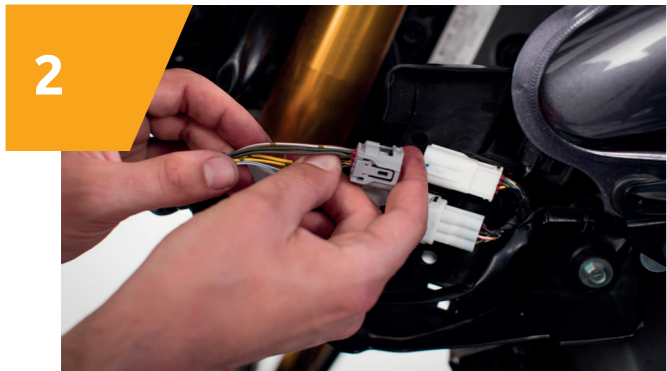
2 Remove main insulation, locate and cut 3 wires (left, right and flasher signal wire), and crimp red bullet connectors. Then locate power supply* (12 V and GND).
