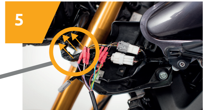
5 Connect remaining 3 ST2 wires (white, brown and purple) with wires going to left handlebar switch (left, right and flasher signal wire).
