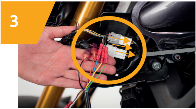
3 Connect power supply* with violet TAB connectors (12 V, GND). Then connect green, yellow and blue ST2 wire with wires going to motorcycle**.
