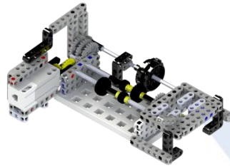
Motor transmission
