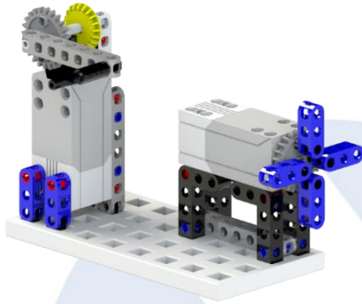
Crank generator
