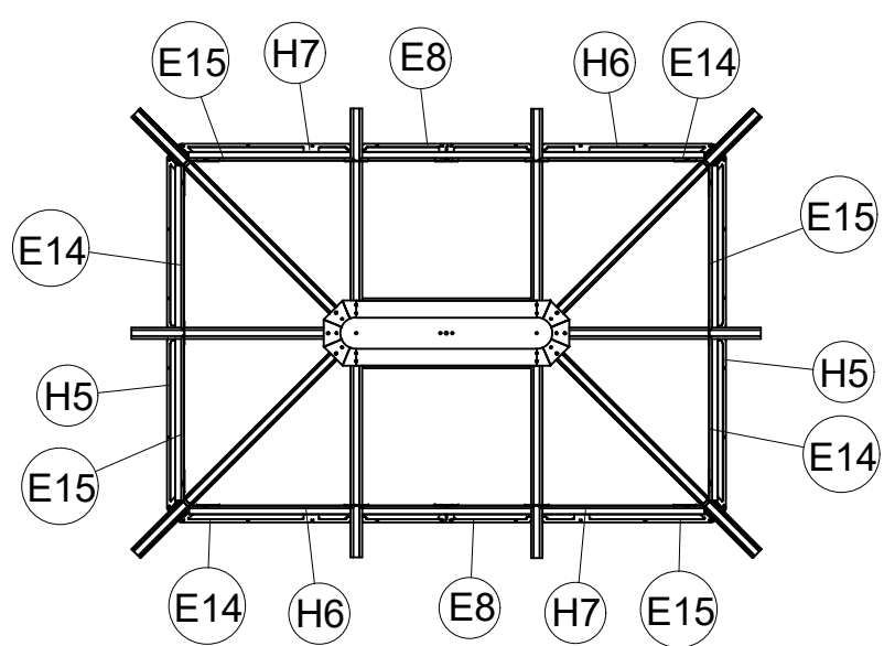
Upward view of the roof
