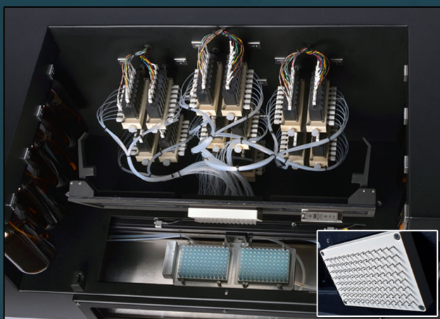
TOP VIEW (INJECTION HEAD DETAIL)
