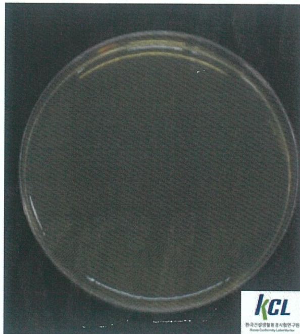
<Picture 2. Escherichia coli - Air Disinfection Purifier (WADU-02) (4 h)>
