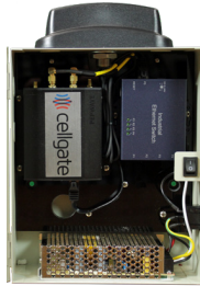
Product includes surface mount flat screen and component NEMA box
