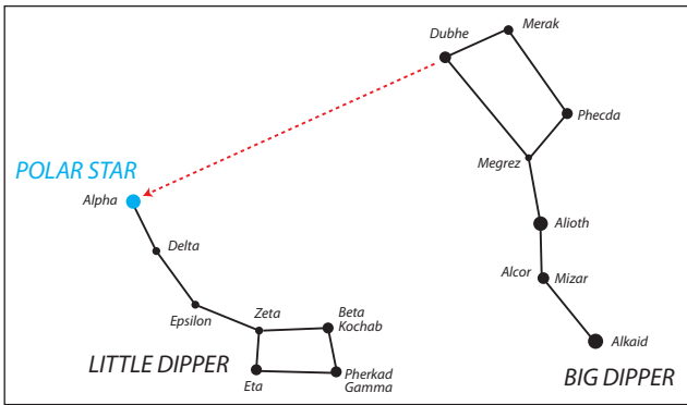
Note: The positioning of the Big Dipper in relation to the Little Dipper does not change, but the orientation of both in the night sky will rotate throughout the year due to the motion of the Earth.
