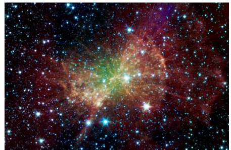
Image credit: NASA/JPL-Caltech/Harvard-Smithsonian CfA
