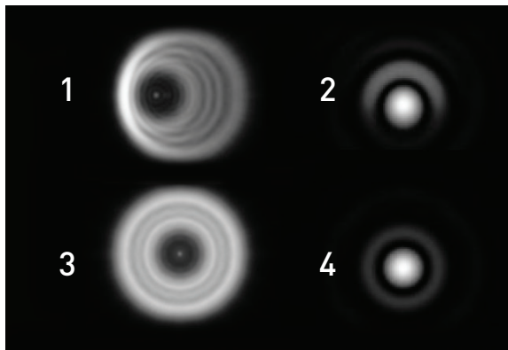
Defocused and focused out-of-collimation star images (1 and 2)
