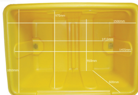
PSB3 INTERNALS
