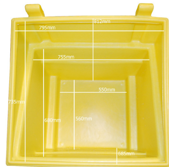
GPSC2 INTERNALS
