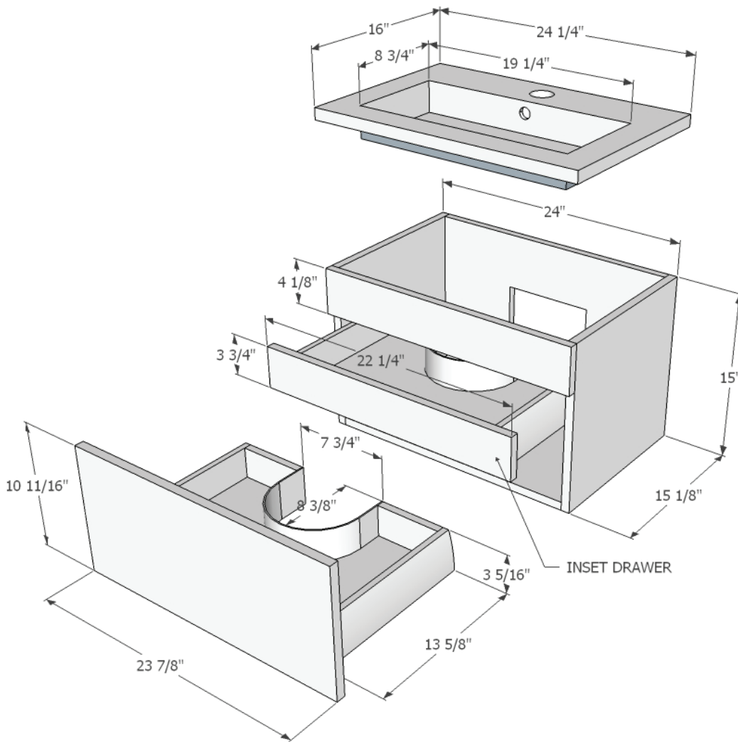
SINK DETAIL
