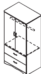
FTTD32W2RA 32"W x 24"D x 72"H or FTTD36W2RA 36"W x 24"D x 72"H
