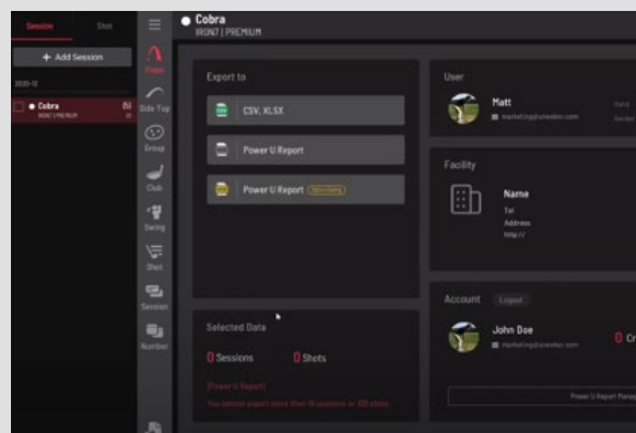
Logged-In Image
