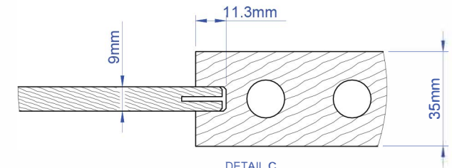
DETAIL C SCALE 1 : 2
