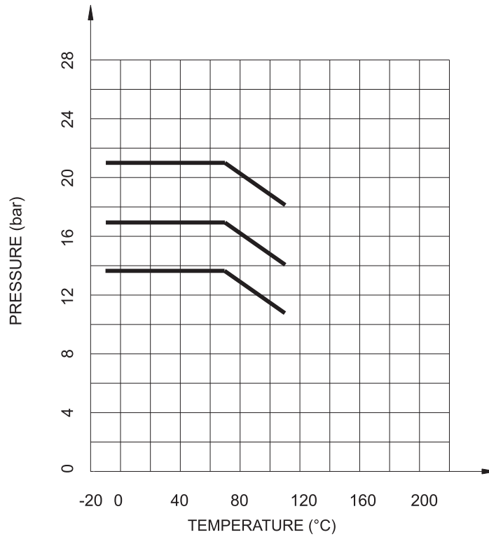
Pressure-Temperature Chart
