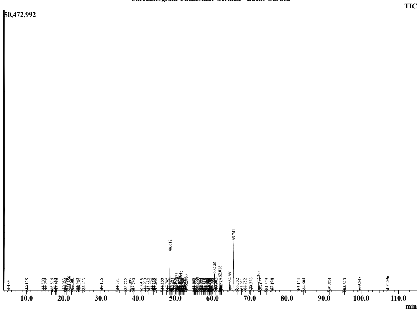
Chromatogram Chamomile German - Edens Garden
