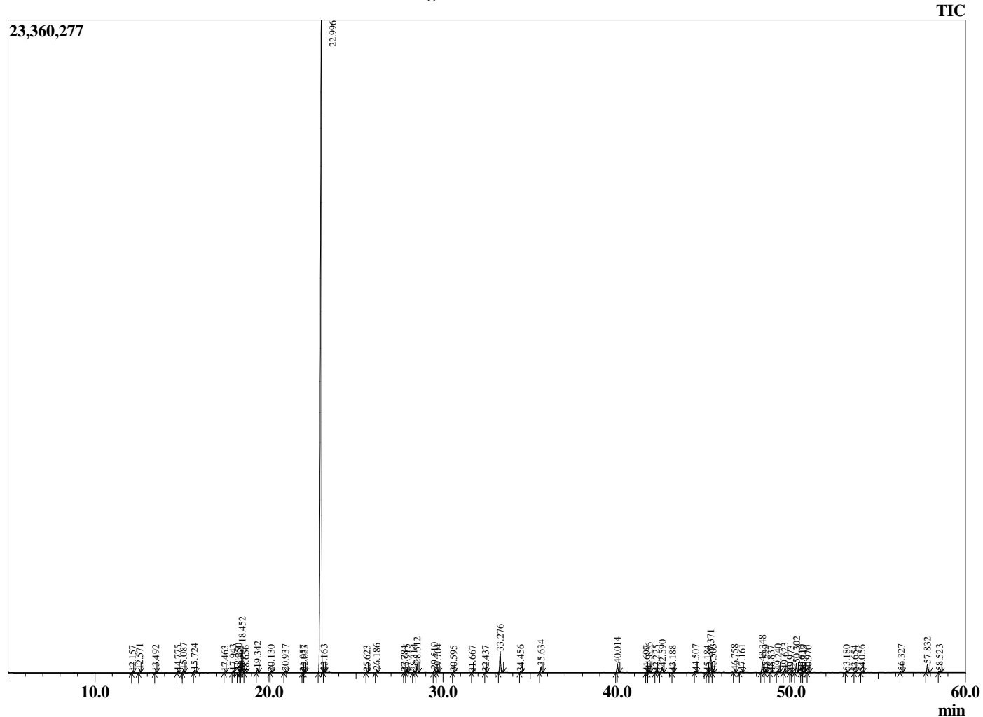
Chromatogram Basil - Edens Garden
