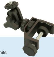
'V' Mount Pole Clamp Large: 16 - 40 mm clamping width
