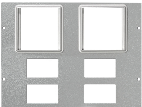
STO279/285 [1][3] 2 x 50mm Euro Module & 4 x LJ6C Data Plate
