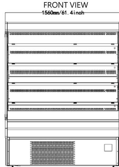
FRONT VIEW 1560mm/61.4 inch
