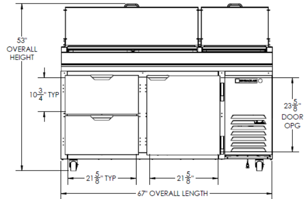
Elevation View
