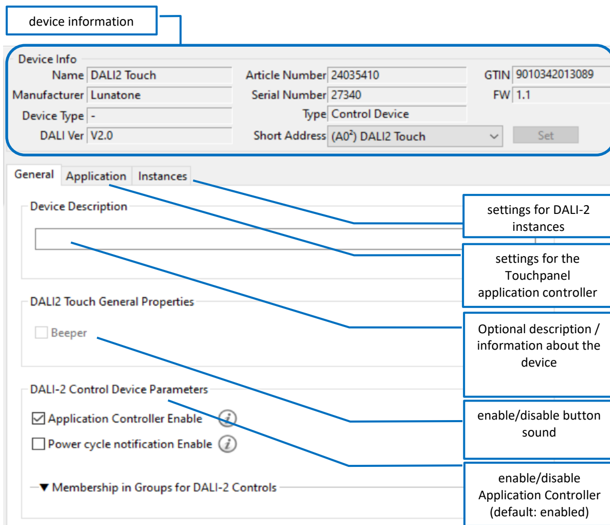
Fig.7 general settings – DALI Cockpit
