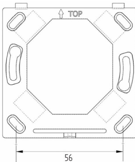
Fig. 3. mounting plate
