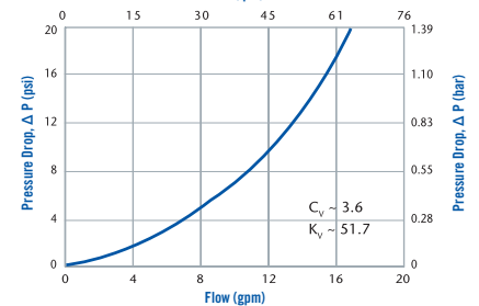
DRUMQUIK PRO & DRUMQUIK PUR WATER FLOW Performance with Pump Suction
