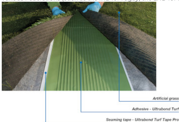
Fig.1 - Bonding system made up of 3 elements: artificial grass, seaming tape and adhesive.
