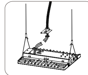
4. Wiring as required and taking safety precautions
