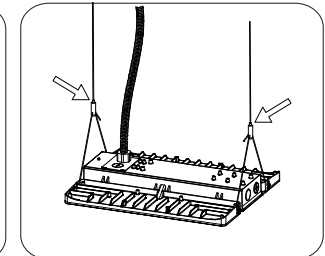
6. Press this button to adjust to the required length and complete the installation
