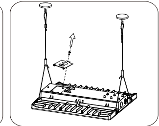
3. Remove the screws and remove the cover
