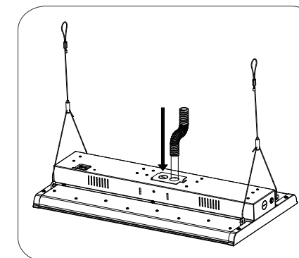
5. Insert the conduit connector and wires into the driver box.
