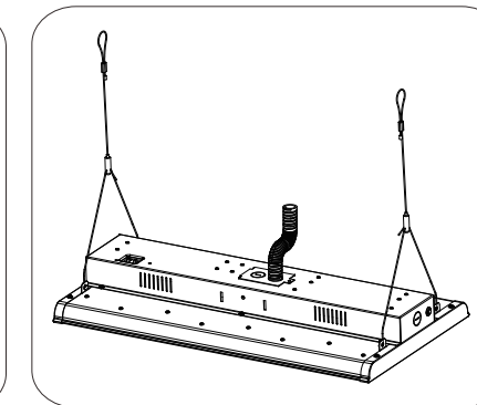
6. Fasten the conduit connector to the wire entry plate.
