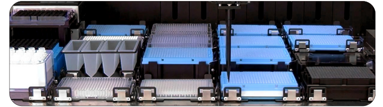
8 Tip Varispan for tube to plate reformatting
