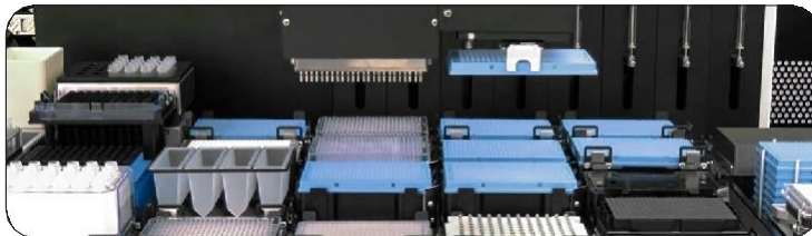
96/384 main array pipettor and labware gripper
