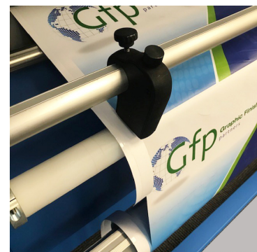
INLINE ROTARY SLITTERS trim the sides of output during lamination to save time and increase productivity.
