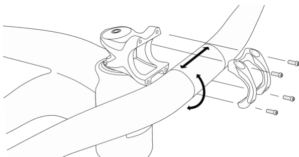
Figure 5.1 Mountain Handlebar Installation
