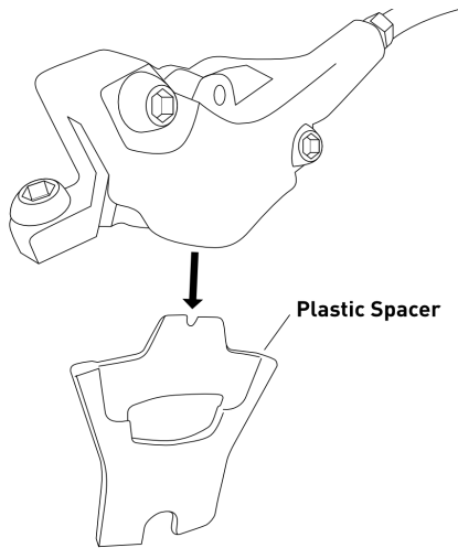
Figure 11: Brake Pad Spacer
