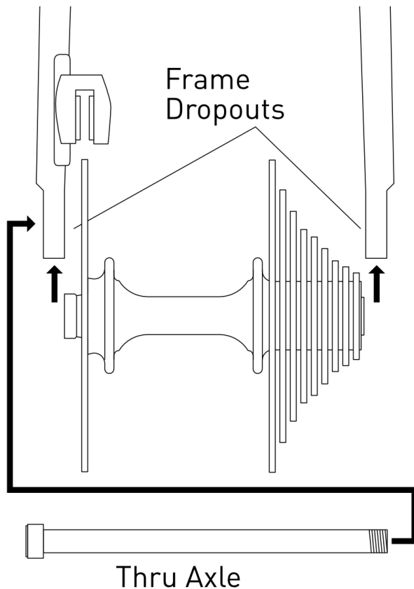
Figure 9: Rear Thru-Axle Installation
