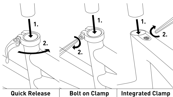
Figure 14 - Seatpost Installation
