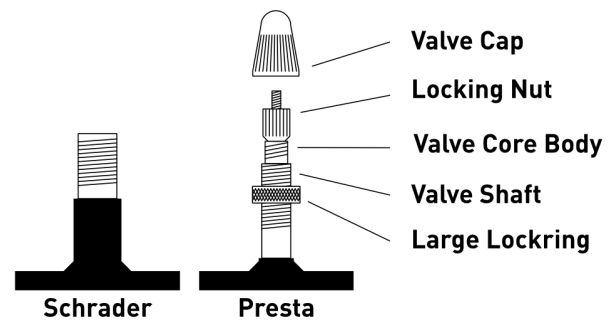
Figure 17: Tire Valve Types
