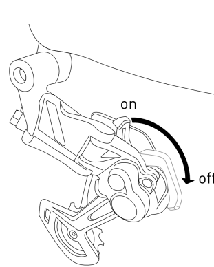
Lever type clutch
