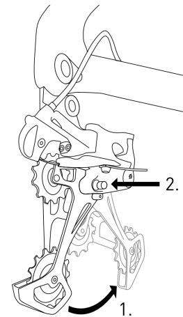
SRAM clutch
