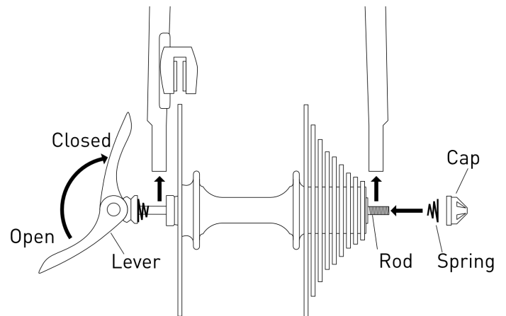
Figure 10: Rear Quick-Release Installation
