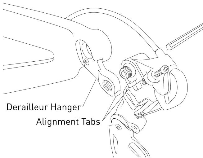
Figure 6: Derailleur Installation
