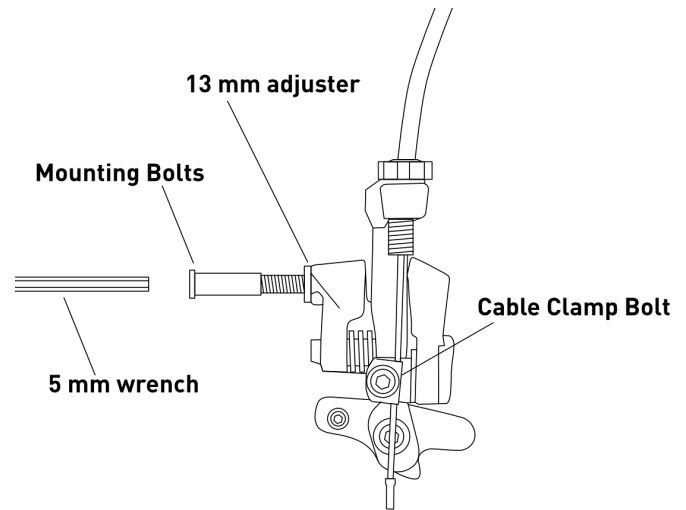
Figure 19 - Rim Brake Adjustments
