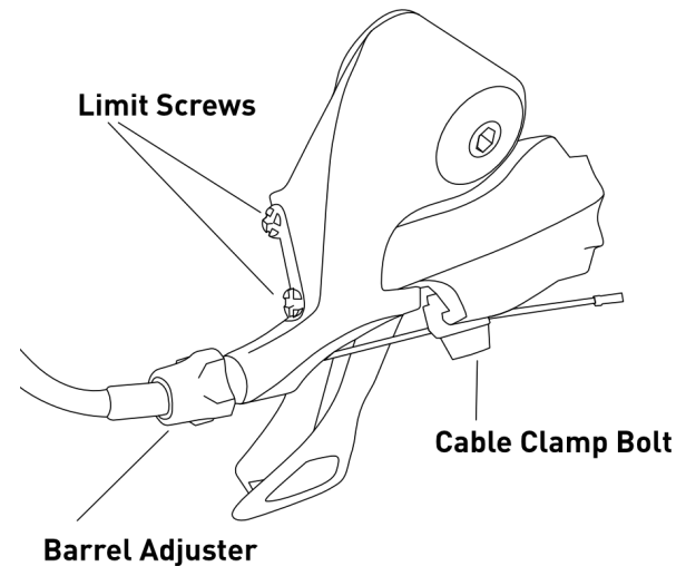
Figure 21 - Rear Derailleur Adjustments
