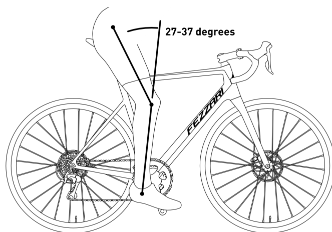
Figure 15 - Seat Height Position
