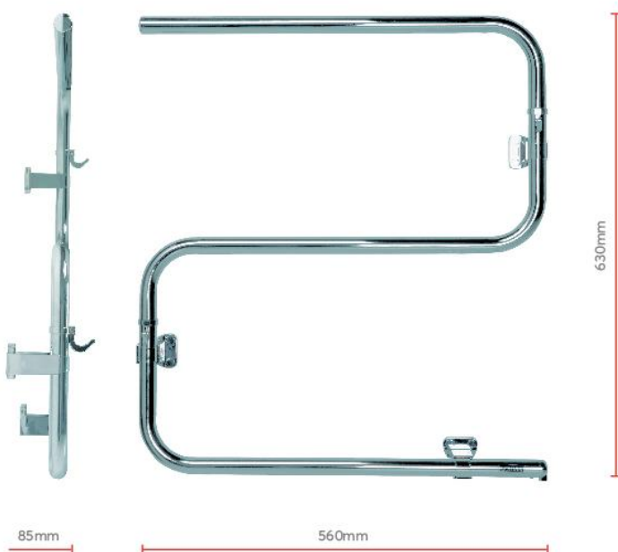
Product dimensions
