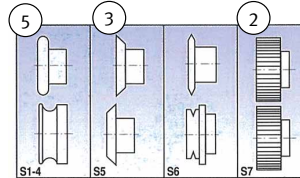
S1-4: Standard rollers for \varnothing 3/6/8/10 mm
