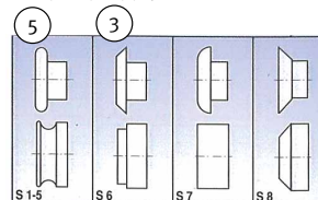
S1-5: Standard rollers for \varnothing 4/6/7/9/10 mm
