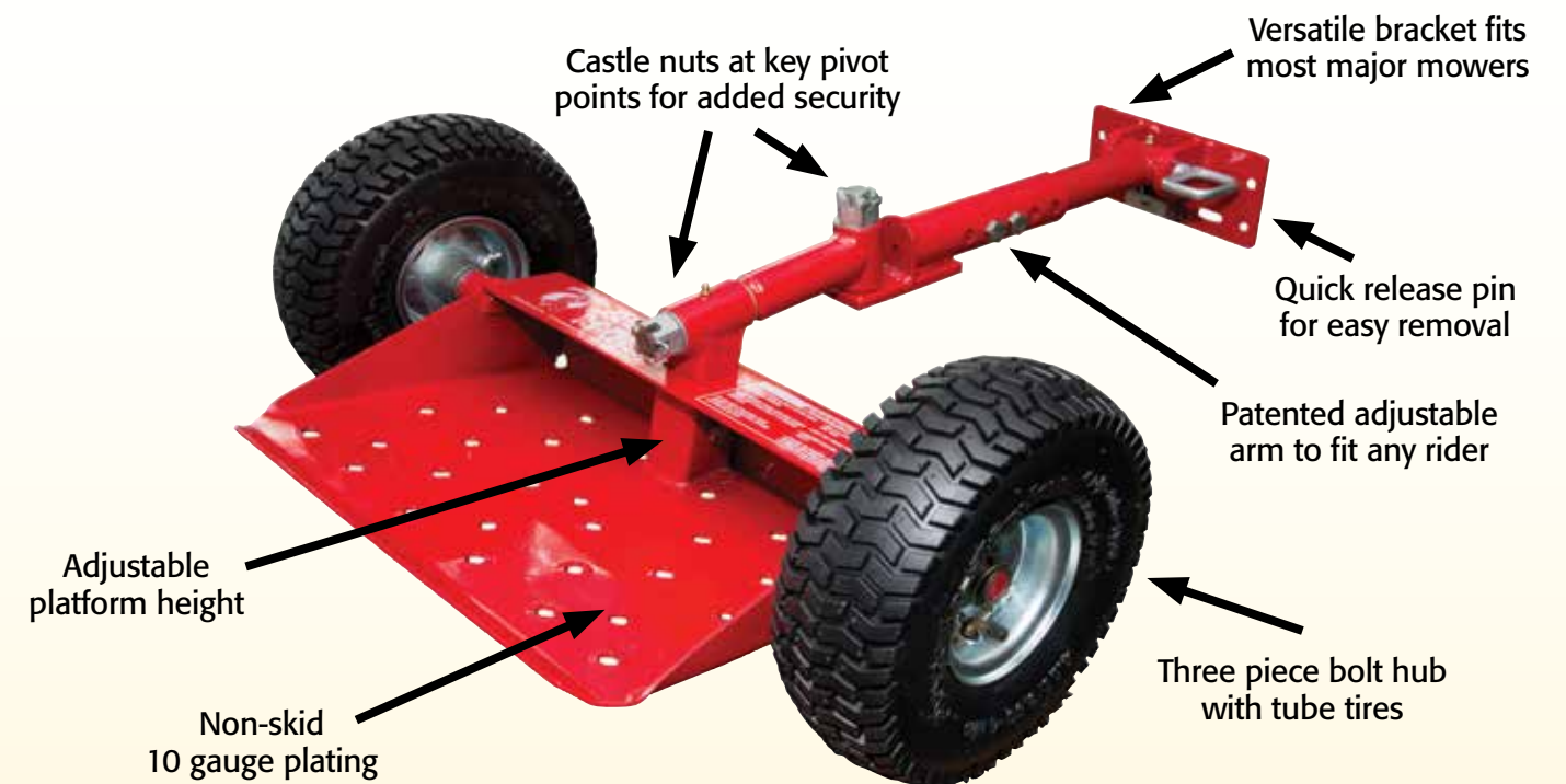
Jungle Wheels - Item # JW BLACK or JW RED
