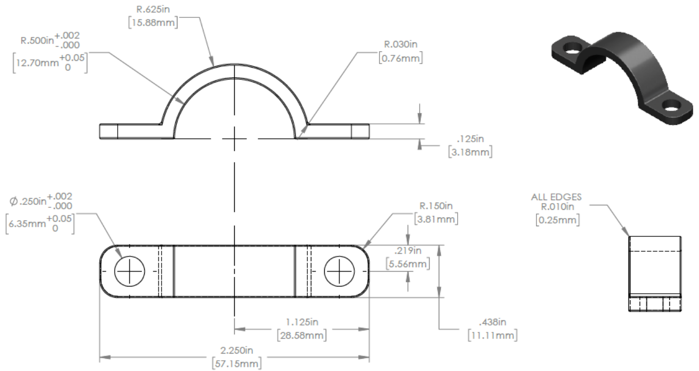
Figure 10 Upper Rack Mount
