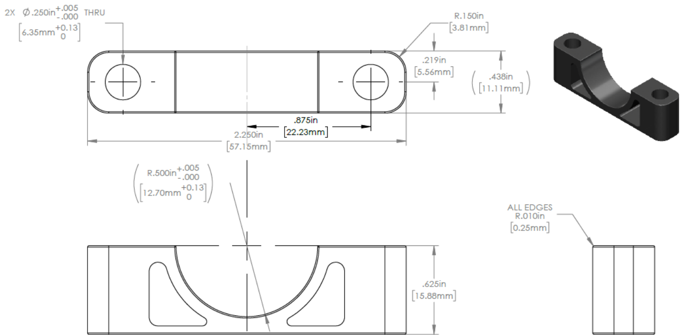
Figure 10 Upper Rack Mount
