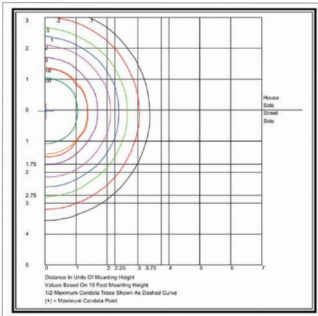
Model AEISAL187-F-1X-302-UNI-5K-CL (302W)
