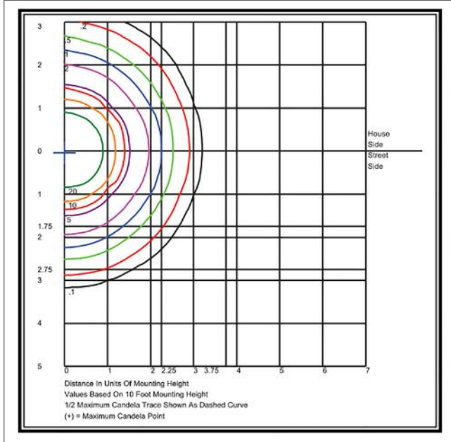
Model AEISAL187-F-1X-187-UNI-5K-CL (187W)
